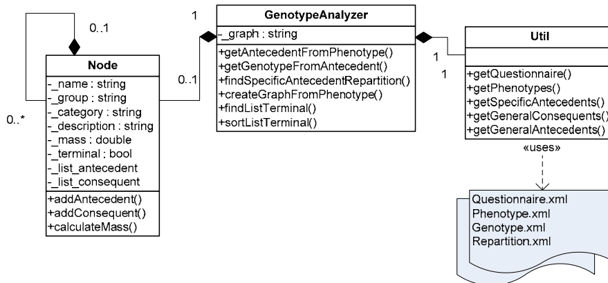
Figure 2 Our UML diagram for modeling consequent-antecedent links
