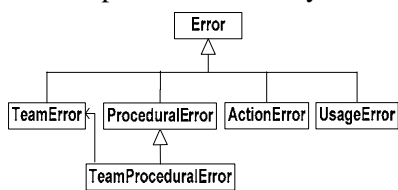
Figure 1a. Errors types in ITS (Buche and Querrec, 2005)
