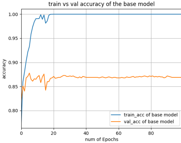
Fig. 4. Training vs validation accuracy of the base model
