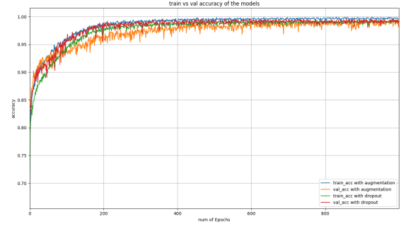
Fig. 5. Training vs validation accuracy of the models
